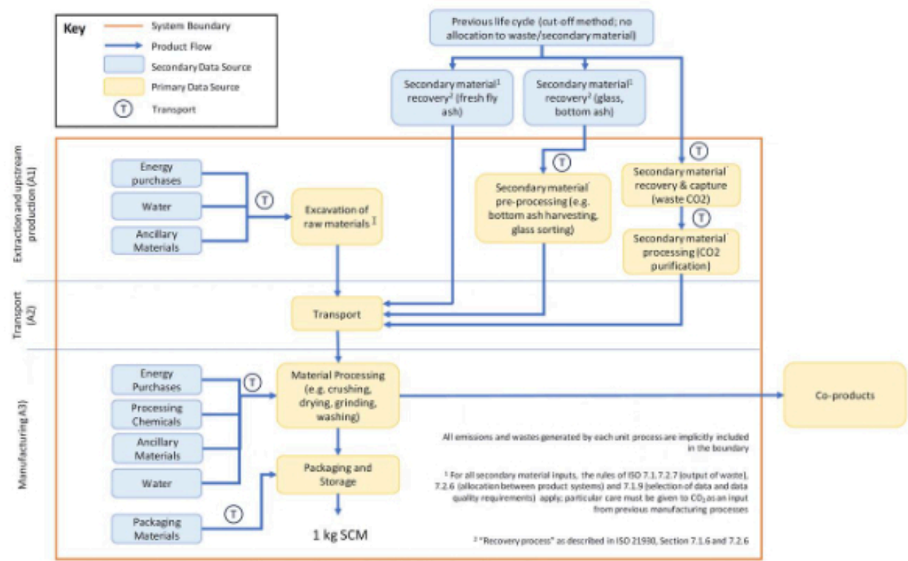
Figure 2. Example SCM System Boundary
