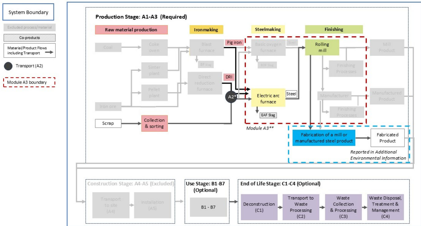
Figure 1. Product Flow Diagram
